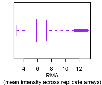
c) Boxplot
