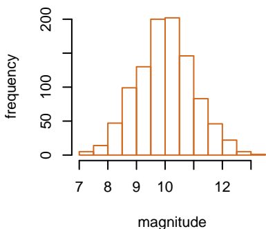
d) Histogram
